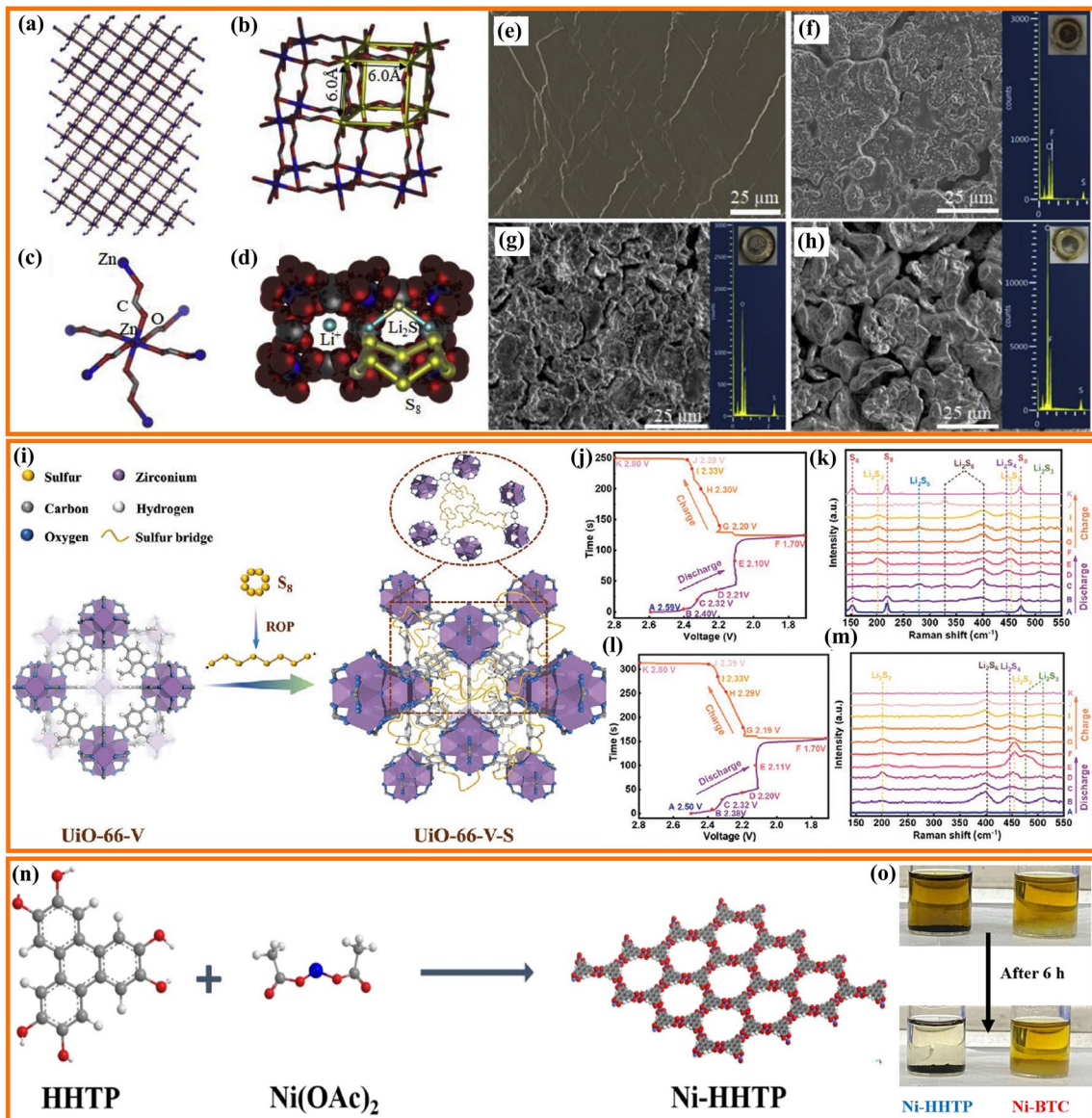
Fig. 19 Crystal structure representation of the 3D network DMAZF, where a crystal structure packing. b Size of the network window into the void space. c Metal node displaying the carbon and oxygen coordination to Zn. d Description of the LiPS mitigation process and the entry of Li ions through the nanopores. e Surface morphology of the uncycled anode of DMAZF/CNTs/sulfur electrode. f Cycled anode in the presence of DMAZF/CNTs/sulfur electrode. The surface morphology of the cycled anode g Br-UIO-66/CNTs/sulfur electrode and h UIO-66/CNTs/sulfur electrode [271]. Copyright 2020, Elsevier. i Schematic diagram of the preparation of UiO-66-V-S. j Voltage–time curves of UiO-66-V/S cathode. k In situ Raman spectra of UiO-66-V/S cathode. l Voltage–time curves of UiO-66-V-S cathode. m In situ Raman spectra of UiO-66-V-S cathode [258]. Copyright 2022, Wiley-VCH. n Schematic illustration of the fabrication of Ni-HHTP. o Polysulfides adsorption experiment of Ni-HHTP and Ni-BTC [272]. Copyright 2021, Elsevier
