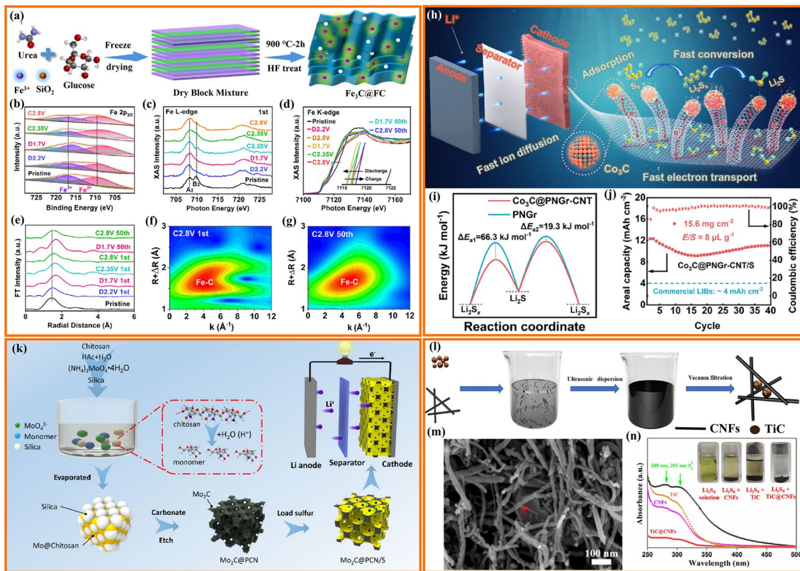
Fig. 17 a Diagram of the synthesis of Fe 3 C@FC composites. b Fe 2p 3/2 XPS spectra. c Fe L-edge XANES spectra. d Fe K-edge XANES spectrum and e corresponding FT-EXAFS spectra of Fe 3 C@FC/S-CF at different states of charge. WT transform contour plots of Fe K-edge after f 1 cycle and g 50 cycles [241]. Copyright 2022, Elsevier. h Schematic diagram of the Co 3 C@PNGr-CNT bidirectional catalytic conversion of LiPS. i The activation energy ( E_a ) of the deposition and decomposition of Li 2 S. j Cycling performance of Co 3 C@PNGr-CNT/S cathode with a high-sulfur loading and a relatively low E/S ratio [242]. Copyright 2022, Elsevier. k Illustration of the fabrication of the Mo 2 C@PCN/S [249] Copyright 2022, Elsevier. l Schematic illustration for the fabrication of TiC/CNFs. m SEM image of TiC/CNFs. n UV-Vis spectra and digital photographs (inset) of Li 2 S 6 solution before and after adding CNFs, TiC and TiC/CNFs [243]. Copyright 2022, Springer Nature
