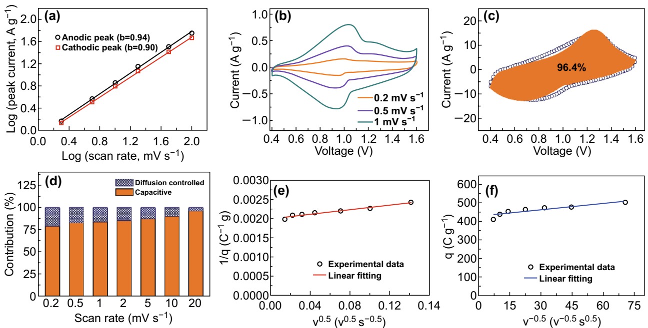
Fig. 4 Kinetic analysis of Zn^{2+} storage in the RuO_2 \cdot H_2O : a relationship curve of peak current versus scan rate, b CV curves at low scan rates of 0.2–1 mV s^{-1} , c capacitive contribution (orange region) to the total current at 20 mV s^{-1} , d summary of the contribution ratios of capacitive capacity and diffusion-controlled capacity, e , f capacitive contribution analyzed through Trasatti’s method, in which q and v are charge stored and scan rate, respectively
